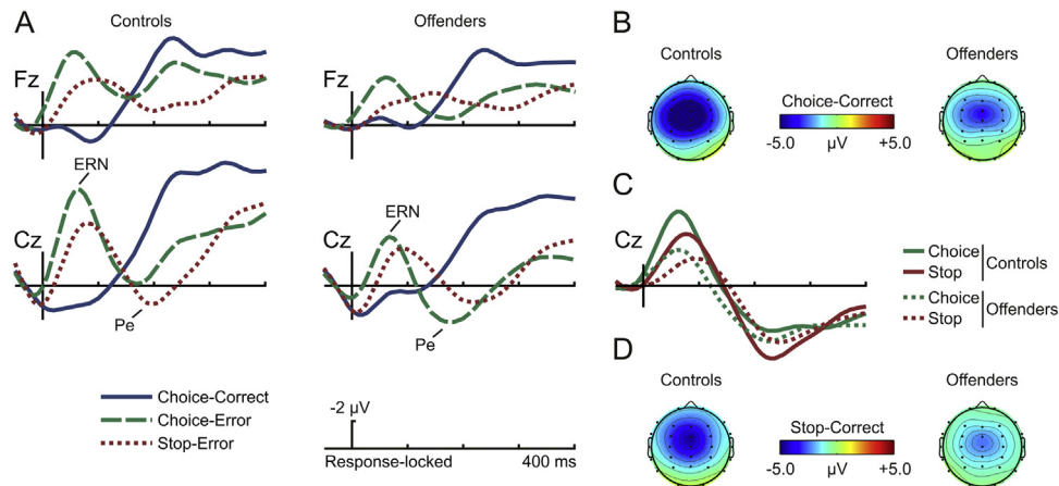
Fig. 2. (A) Grand average of the response-locked ERPs at the midline electrodes in the control and juvenile non-psychopathic violent offender groups [correct trials (solid lines), choice-error trials (dashed lines) and stop-error trials (pointed lines)]. For illustration purposes, these averages were low-pass filtered (lowpass filter, 12 Hz). (B). Scalp distribution for choice-error vs. choice-correct subtraction for the time window 35–85 ms and for the control and offender groups (minimum and maximum values, -5.0/+5.0 \mu\text{V} ). (C) ERPs for choice-error and correct difference, and for stop-error and correct difference, at the Cz electrode for the control (solid lines) and offender (pointed lines) participants. (D) Topography for the subtraction between the stop-error vs. choice-correct conditions for the time window of 65–115 ms for the control and offender groups (min. and max. amplitude values, -5.0/+5.0 \mu\text{V} ).
