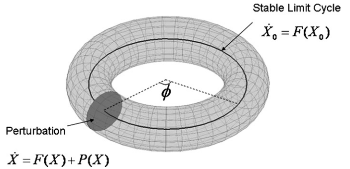
Fig. 1. Phase reduction. The solid circular line shows the state space X_0 of a system on a limit cycle. The limit cycle is assumed stable so that after a small perturbation, the system returns to X_0 . Although X_0 may be high-dimensional the state will be uniquely determined by its position around the orbit, or the 'phase', \phi(X_0) . The dynamics of perturbed solutions are constrained to the space X shown by the torus. The solid disc corresponds to an 'isochron', meaning that all points on this disc have the same asymptotic phase. Using this notion, as we show in the main text, the high-dimensional state equation can be reduced to the one-dimensional system \dot{\phi} = f + z(\phi)p(\phi) . This is known as a phase reduction .
